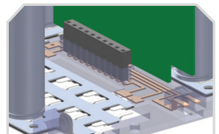
Female receptacle connects control board to overmolded lead frame male connector
