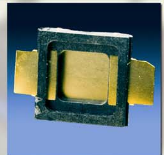
Single Stage LDMOS Amplifier Package
