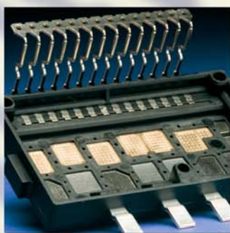
Motor Driver Power Amplifier
