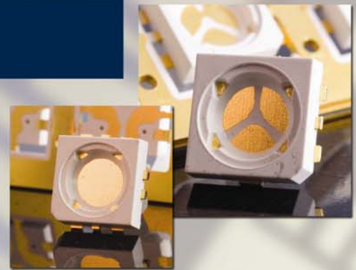
Parallel (Multicolor) LED Package
