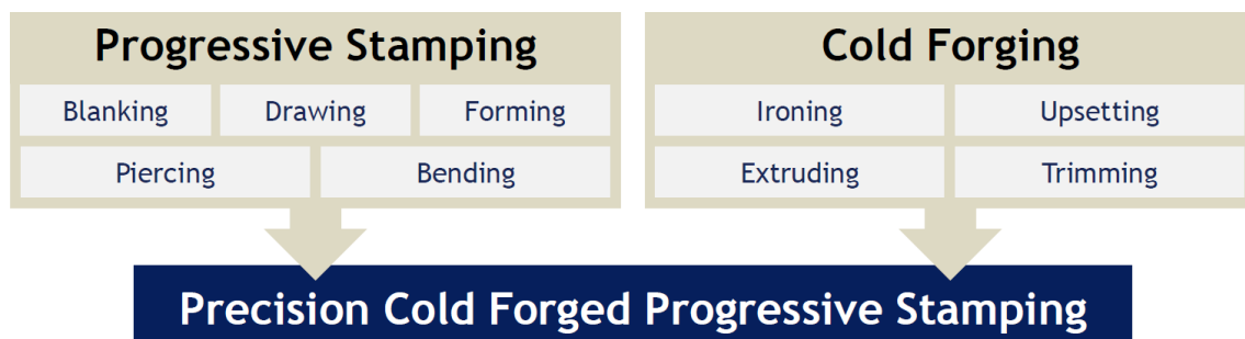
Figure 3 – Precision Cold Forged Progressive Stamping Leverages a Blend of Complementary Processes
