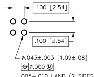
3 RECOMMENDED PRINTED CIRCUIT BOARD HOLE CONFIGURATION
