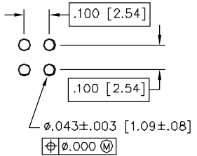
RECOMMENDED PRINTED CIRCUIT BOARD HOLE CONFIGURATION
