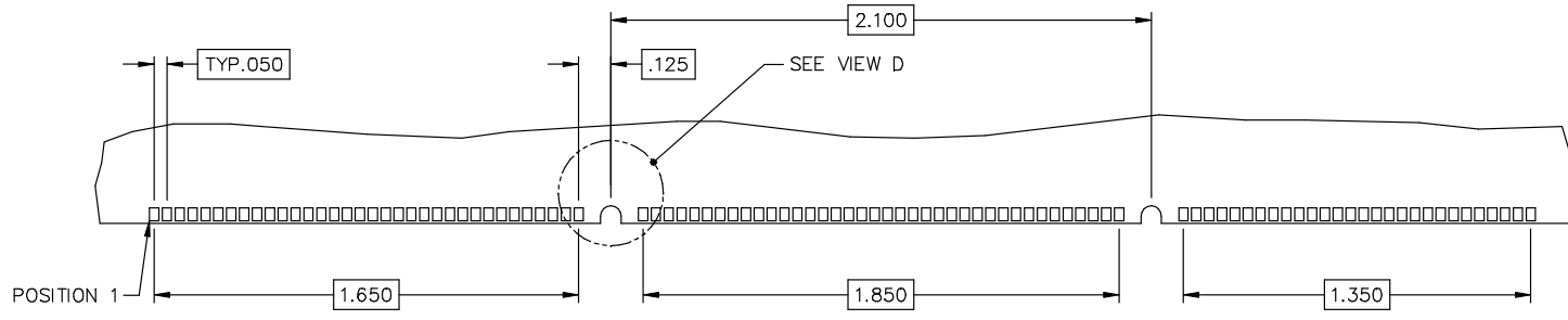
RECOMMENDED DAUGHTER CARD LAYOUT (2 SIDES)
