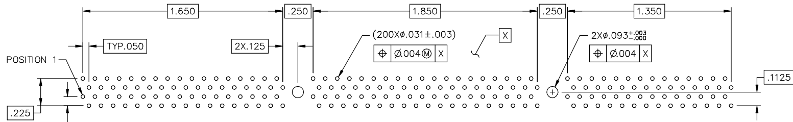
RECOMMENDED HOST CARD LAYOUT - COMPONENT SIDE
