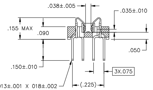
TYPICAL SECTION A-A SCALE = 4:1 (RETENTION POST OMITTED)
