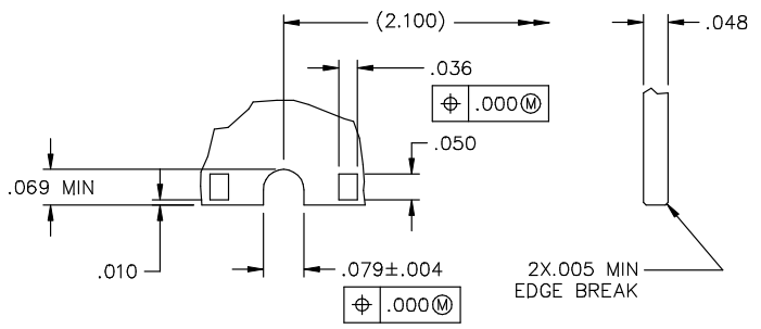
VIEW D - TYPICAL PAD AND KEY SLOT DETAIL SCALE=4:1
